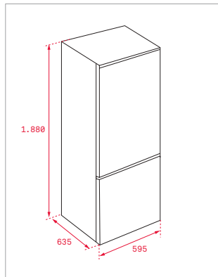
NFL 345 C - NFL 342 C - NFL 320 C NFL 320
