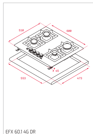
EFX 60.1 4G DR
