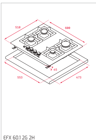
EFX 60.1 2G 2H
